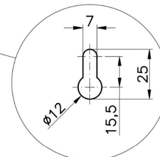
Particolare asole Detail fixing holes
