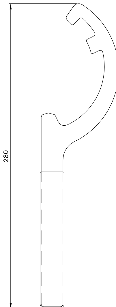
Vista laterale Side view
